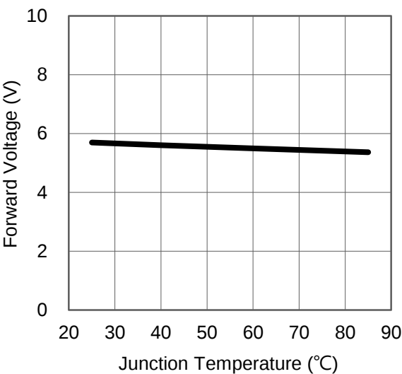
Fig 6. Junction Temperature vs. Forward Voltage
