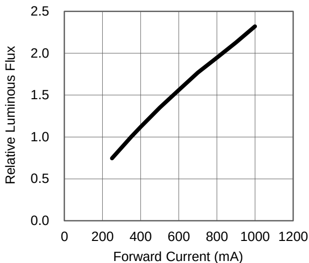
Fig 2. Relative Luminous Flux vs. Forward Current for 2100 K at T_j = 25 maintained.
