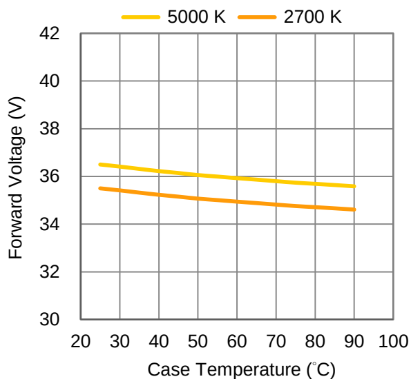
Fig 5. Case Temperature vs. Forward Voltage at 700 mA.
