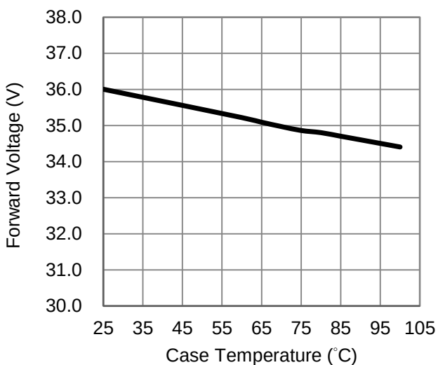
Fig 2. Case Temperature vs. Forward Voltage at 360mA.
