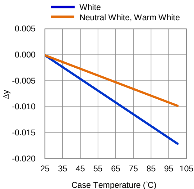
Fig 4. Case Temperature vs. Chromaticity Coordinate \Delta y at 360mA.
