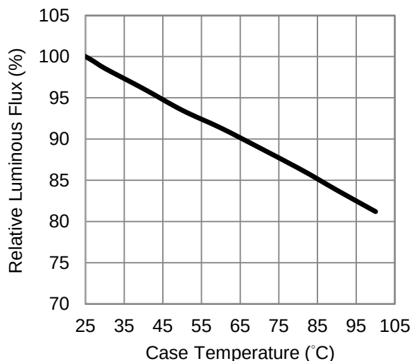
Fig 1. Case Temperature vs. Relative Luminous Flux at 360mA.
