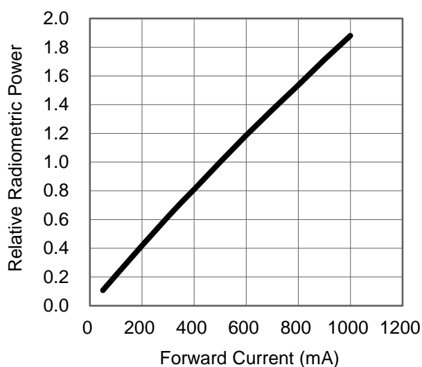
Fig 2. Relative Radiometric Power vs. Forward Current for 365nm + 385nm + 395nm + 405nm at T_j=25 maintained.
