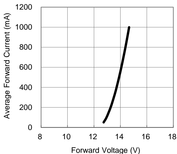
Fig 1. Forward Current vs. Forward Voltage for 365nm + 385nm + 395nm + 405nm.
