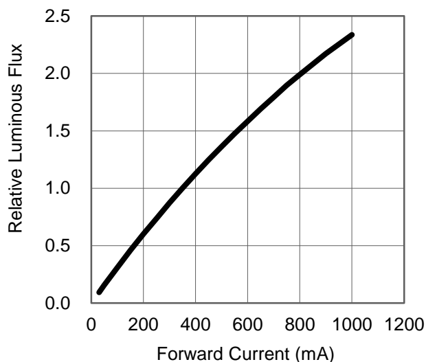
Fig 2. Relative Luminous Flux vs. Forward Current for PC Amber at T_J = 25^\circ\text{C} maintained.
