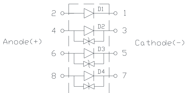
Circuit Diagram
