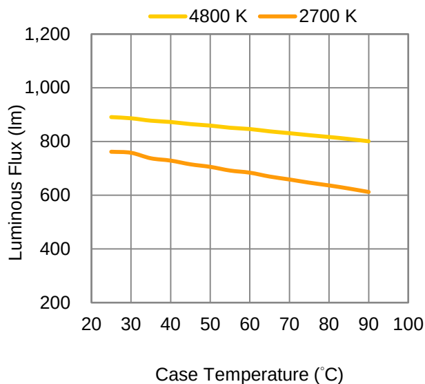
Fig 4. Case Temperature vs. Luminous Flux at 200 mA.
