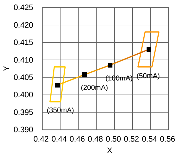
Fig 7. Chromaticity Coordinate Profile at T_C=25^\circ\text{C} .
