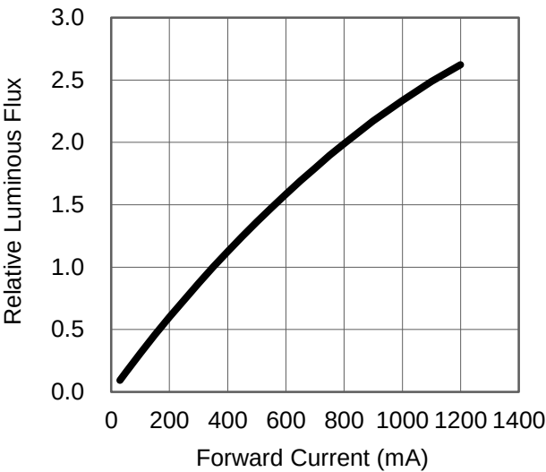
Fig 2. Relative Luminous Flux vs. Forward Current for PC Magenta at T_j=25 maintained.
