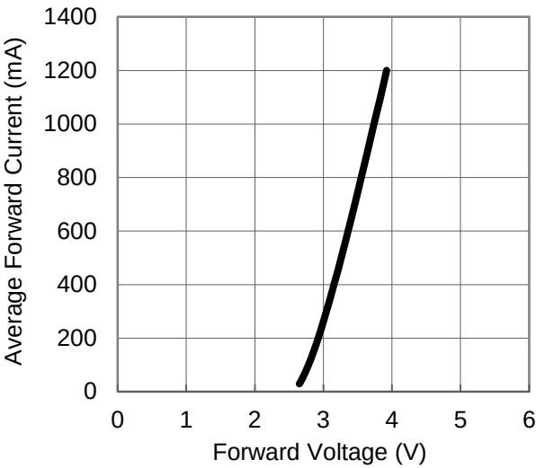
Fig 1. Forward Current vs. Forward Voltage for PC Magenta.
