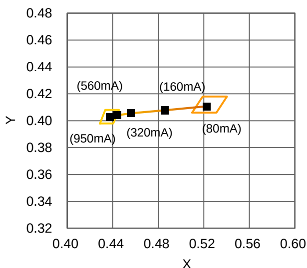
Fig 4. Chromaticity Coordinate Profile at T_C=25^\circ\text{C} .
