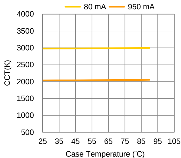
Fig 7. Case Temperature vs. Chromaticity Coordinate \Delta x at 80 mA & 950 mA.
