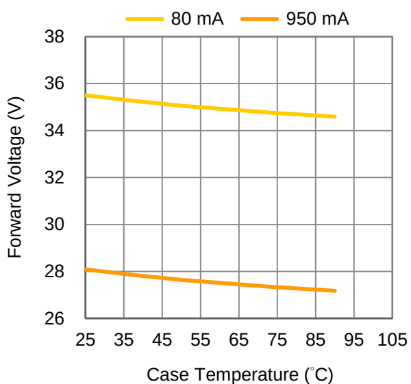
Fig 6. Case Temperature vs. Forward Voltage at 80 mA & 950 mA.
