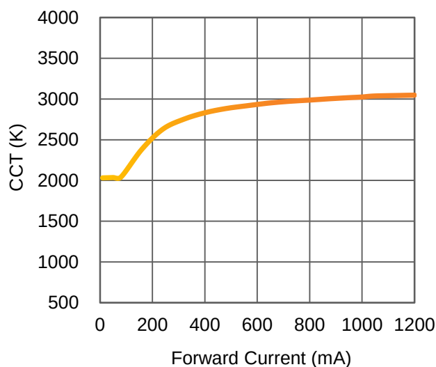
Fig 3. Forward Current vs. Color Temperature at T_C=25^\circ\text{C} .
