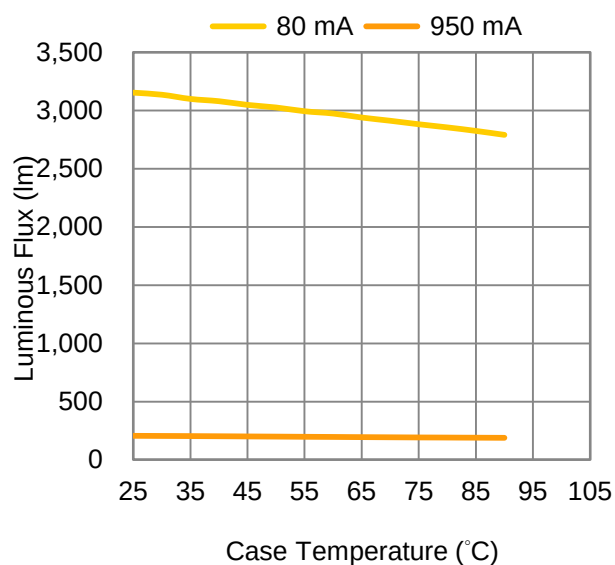
Fig 5. Case Temperature vs. Luminous Flux at 80 mA & 950 mA.
