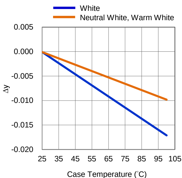
Fig 4. Case Temperature vs. Chromaticity Coordinate \Delta y at 1440mA.
