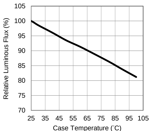
Fig 1. Case Temperature vs. Relative Luminous Flux at 1440mA.
