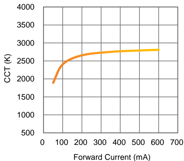
Fig 6. Forward Current vs. Color Temperature at T_C=25^\circ\text{C} .
