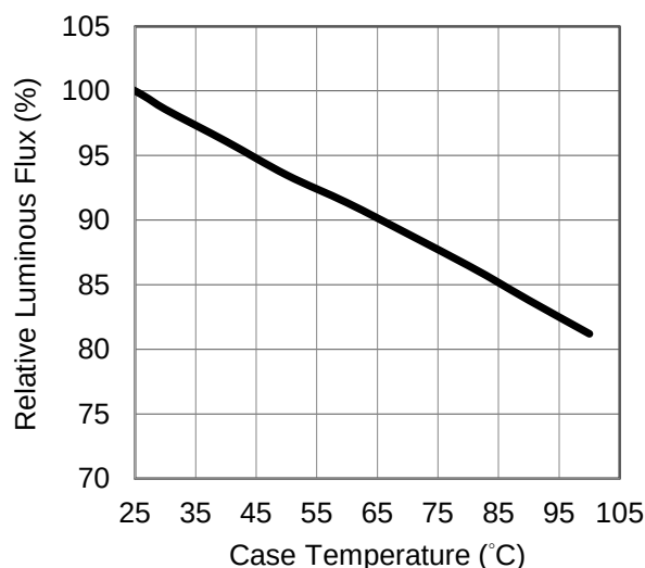
Fig 1. Case Temperature vs. Relative Luminous Flux at 450mA.
