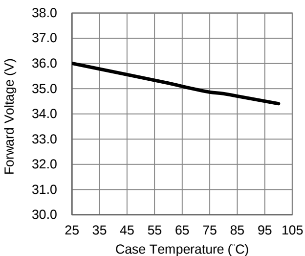
Fig 2. Case Temperature vs. Forward Voltage at 720mA.
