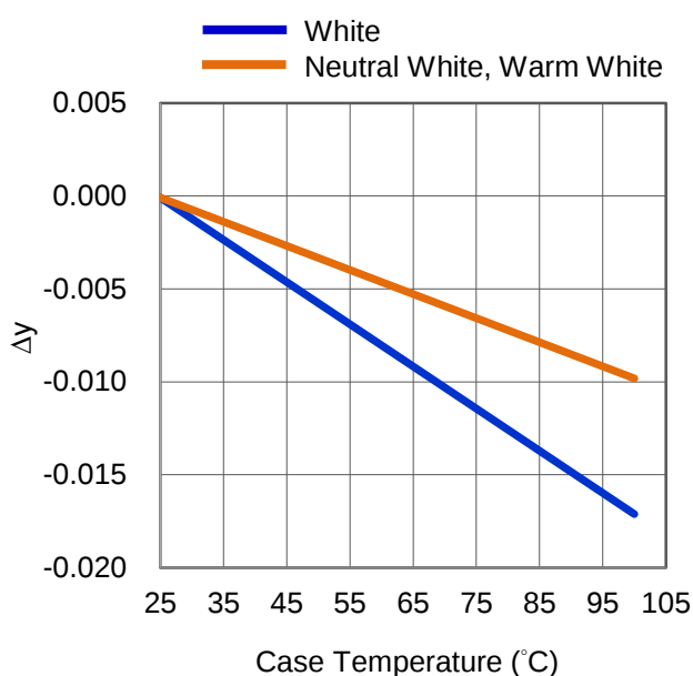
Fig 4. Case Temperature vs. Chromaticity Coordinate \Delta y at 720mA.
