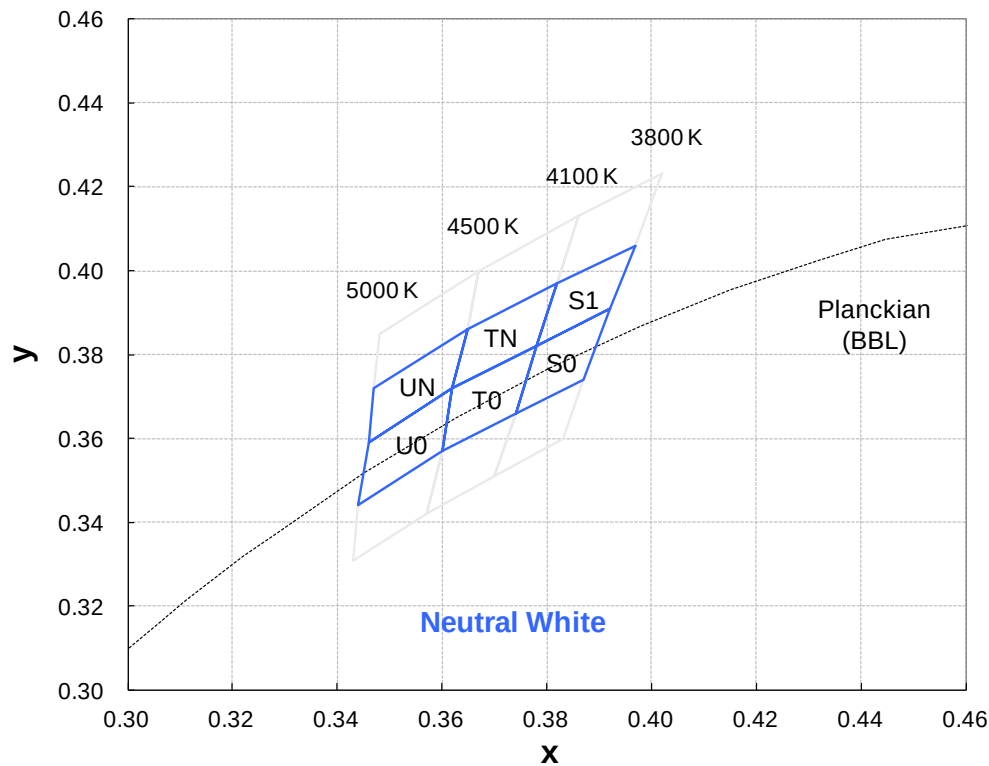
Neutral White Binning Structure Graphical Representation
