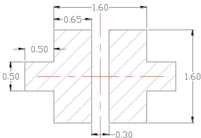
Recommended trace layout : MCPCB
