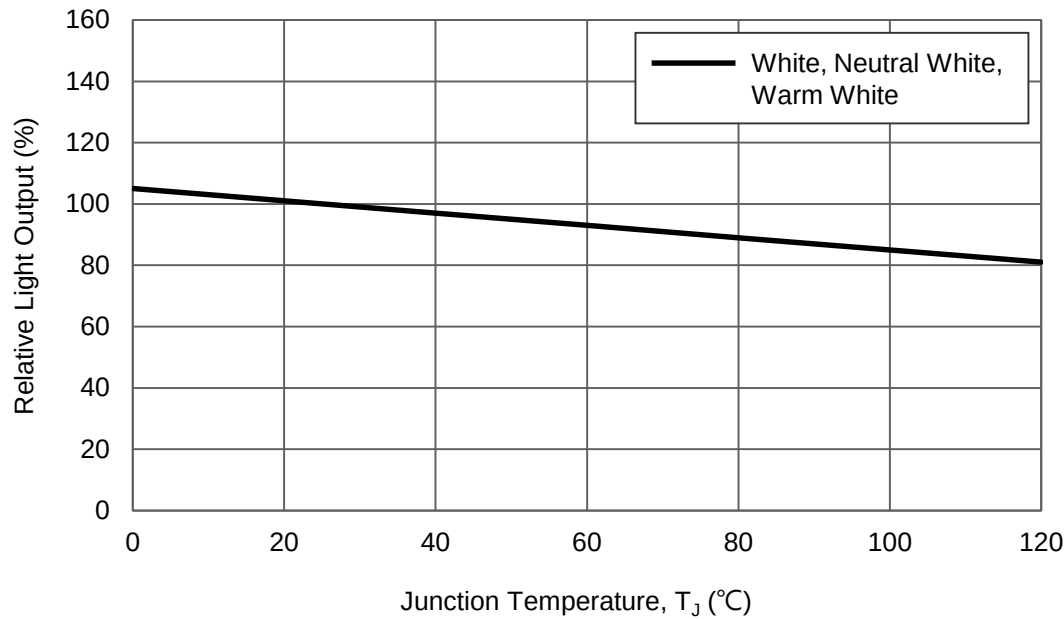
Relative Light Output vs. Junction Temperature at 600mA
