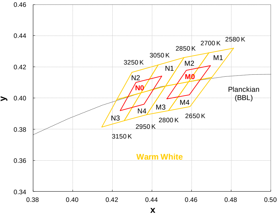
Warm White Binning Structure Graphical Representation
