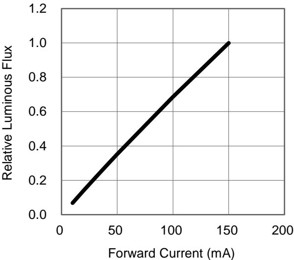
Fig 2. Relative Luminous Flux vs. Forward Current for PC Amber at T_j=25 maintained.
