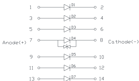
Circuit Diagram
